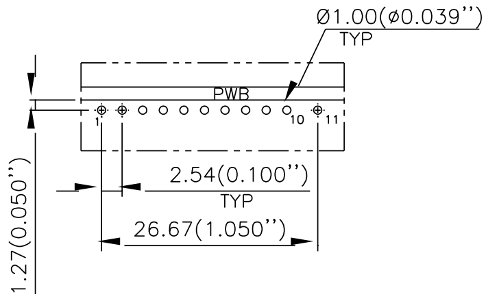
RECOMMENDED PWB LAYOUT
